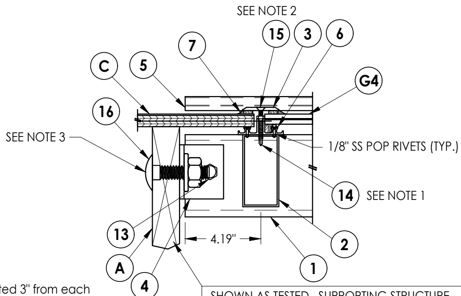
3 CROSS SECTION
