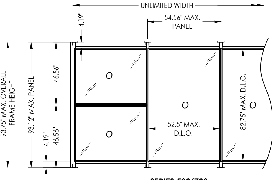
SERIES 500/700 Multi-span
