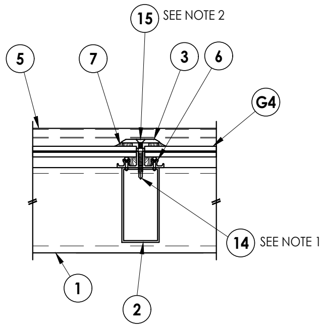
4 CROSS SECTION
